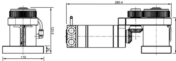
TWIN RIGHT ANGLE DRIVE UNIT
